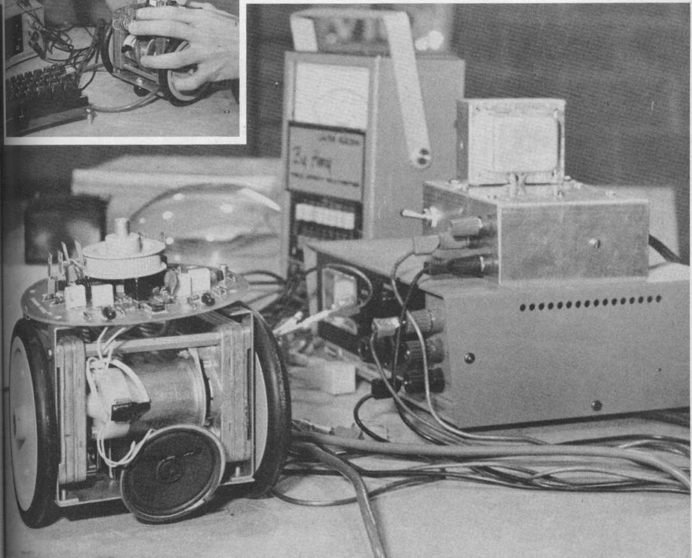
Photo 8: The completed Turtle, connected to a power supply for testing.
