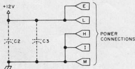
Figure 3: Schematic of the Turtle's touch sensor, lights, and horn control circuitry.
