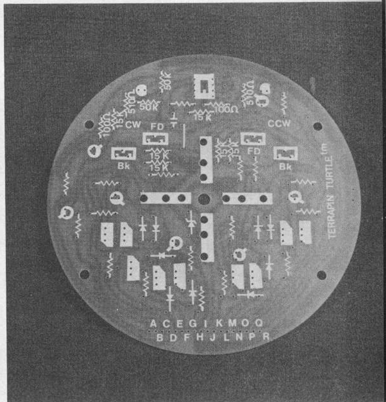
Photo 3: The component side of the circuit board.
